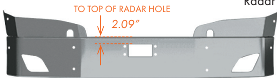
COK-5010-15Z-V6 2 OEM fogs, tow pins, radar Radar requires plastic cover
