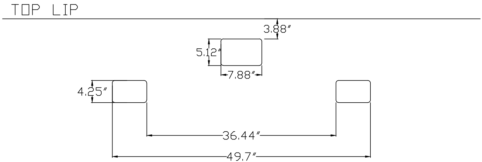
HC STANDARD CUT OUT DIMENSIONS
